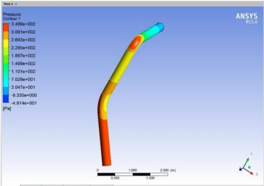
Figure 8. ANSYS pressure contour modeling results
