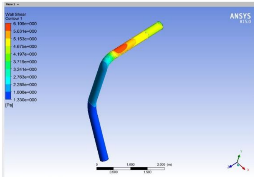
Figure. 9. Results of ANSYS shear stress contour modeling
