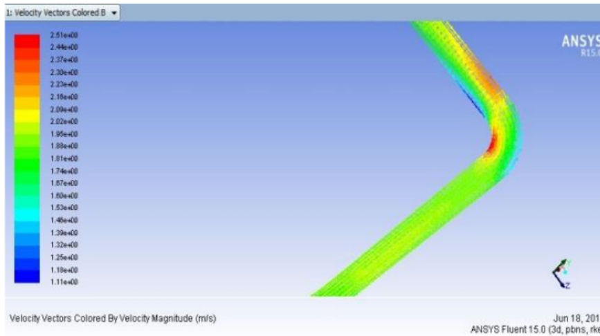
Figure. 10. ANSYS speed vector modeling results
