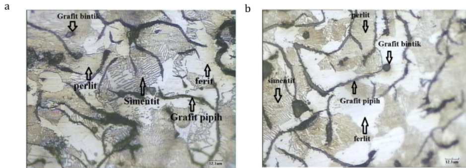
Figure. 6. (a) Cross section after etching magnification 500x; (b) Longitudinal section after etching magnification 500x
