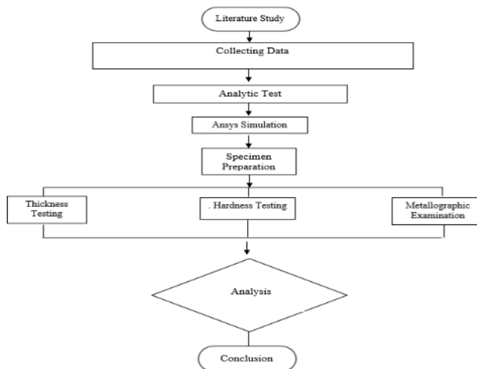
Figure 1. Research Flowchart
