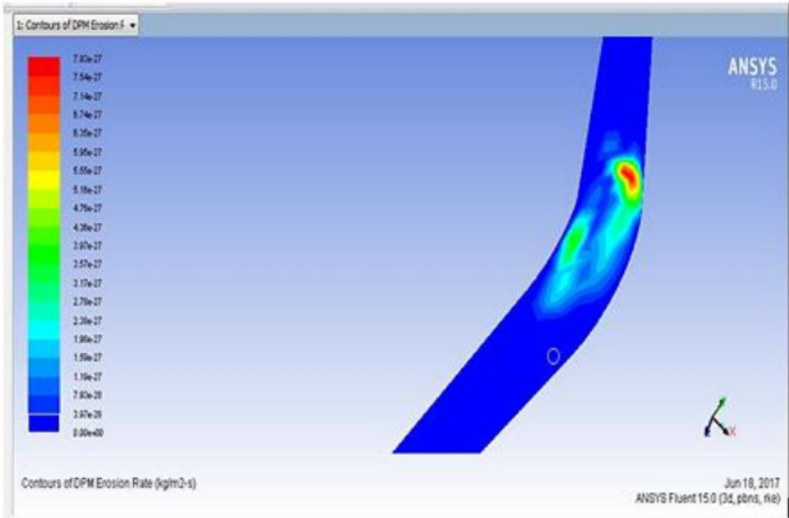
Figure 7. ANSYS erosion corrosion modeling
