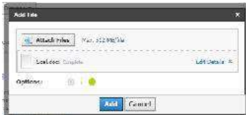
Gambar 61 Attach files
