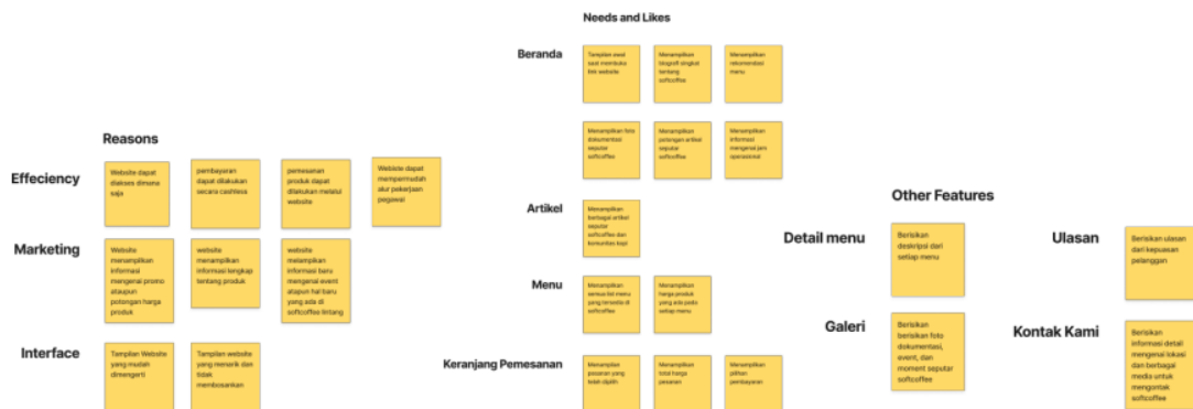
Gambar 3. Diagram Afinitas
