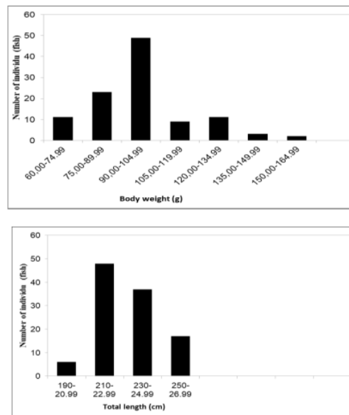
Fig 2: The total length and body weight of Notopterus notopterus (Pallas, 1769) from East Pedamaran Floodplain, Ogan Komering Ilir, South Sumatra, Indonesia
