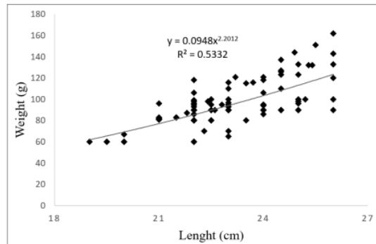
Fig 3: The length-weight relationship of Notopterus notopterus (Pallas, 1769) from East Pedamaran Floodplain, Ogan Komering Ilir, South Sumatra, Indonesia
