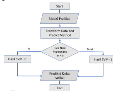
1 Gambar 3. Flowchart Support Vector Regression
