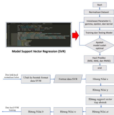
Gambar 2. Model Support Vector Regression
