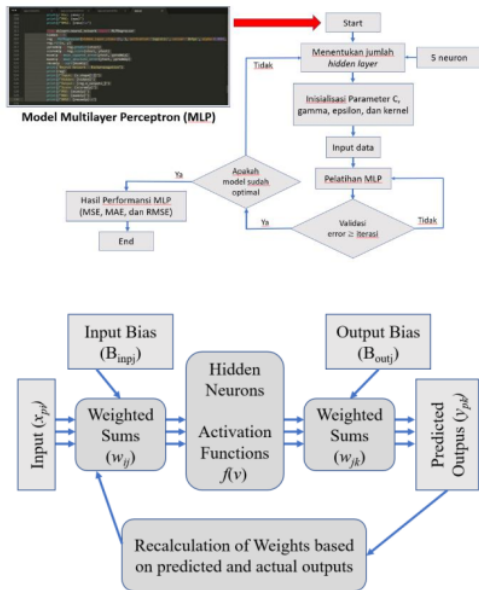
Gambar 4. Model Multilayer Perceptron
