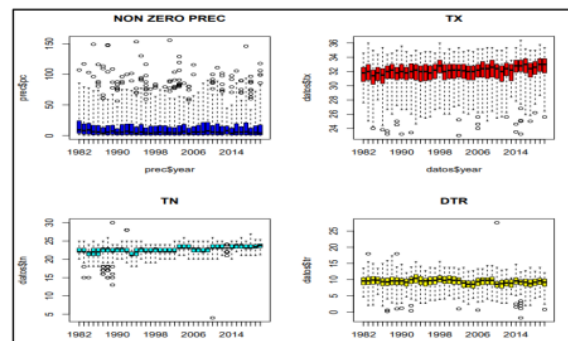
Figure 2. Results of QC analysis for TN, TX, and in SM Japura Rengat 1981-2020
