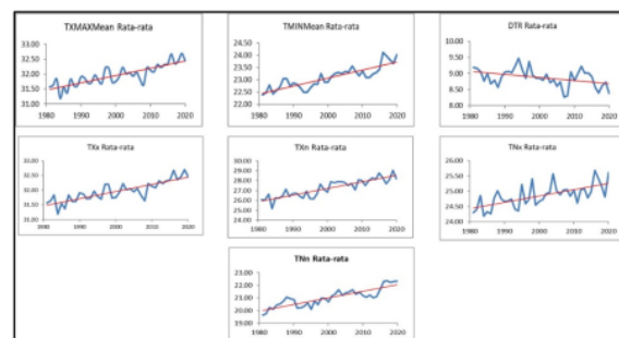
Figure 5. Trend Estimated increase in temperature extreme index over 4 decades (increase per 10 years)
