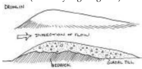
D (Arah deposit glacial tills)
