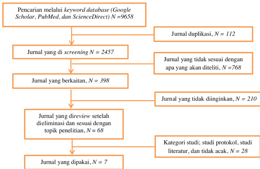
Gambar 1. Alur Prisma
