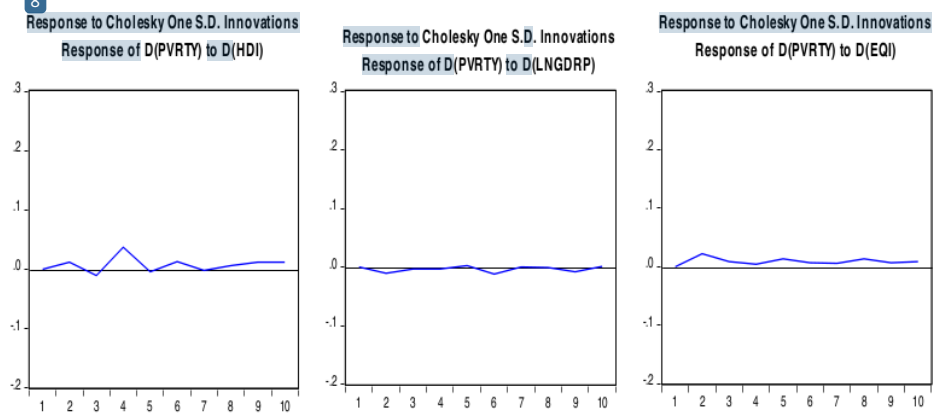
Figure 1. Impulse Response Function
