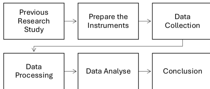
Figure 1. Research Flow
