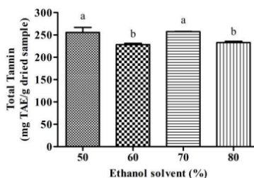
Figure 2. Total tannin content of the extract from N. fruticans fruit husk with different ethanol concentrations. The data are shown as the mean \pm SD ( n=3 ). Different letters above the bars indicate statistically a significant difference at p < 0.05 .
