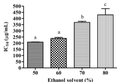
Figure 3. Antioxidant activity of the polyphenol extract from N. fruticans husk with different ethanol concentrations. The data are shown as the mean \pm SD ( n=3 ). Different letters above the bars indicate a statistically significant difference at p < 0.05 .
