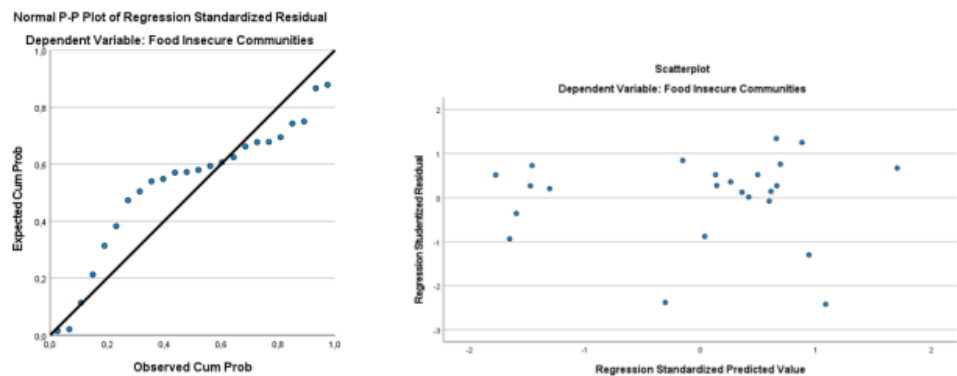
Fig 3. Normality and Heteroskedasity Test
