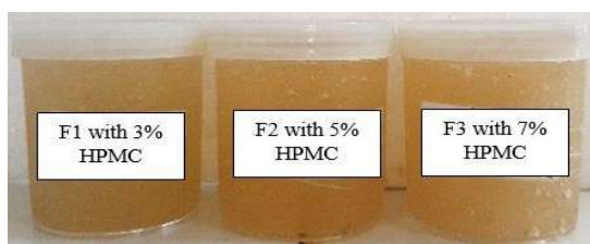
Figure 2. Submicroparticles Gel
