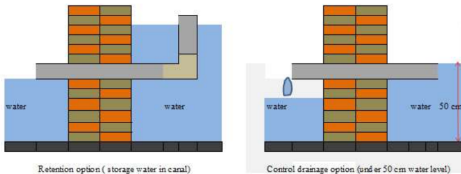
Figure 2. Water level control design in the tertiary canal for the CD option under a 50 cm water level in the tertiary canal of the tidal lowland reclamation area.
