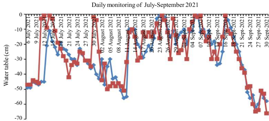
Figure 5. Water table dynamics at the tertiary plot in the tidal lowland of C typology, Telang 1. —♦— : Sampling point 1, —■— : sampling point 2.
