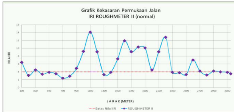
Figure 1. Road surface roughness graph of Alamsyah RPN street from normal direction ( Roughmeter II )
