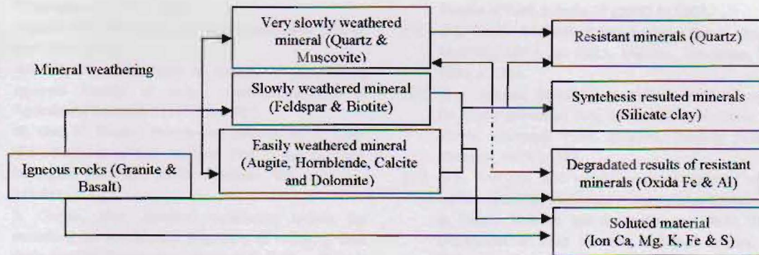
Fig. 2 Rock weathering diagram in acid conditions.
