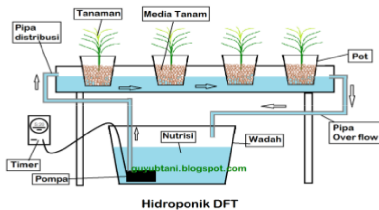
Gambar 38. Deep Flowing System
