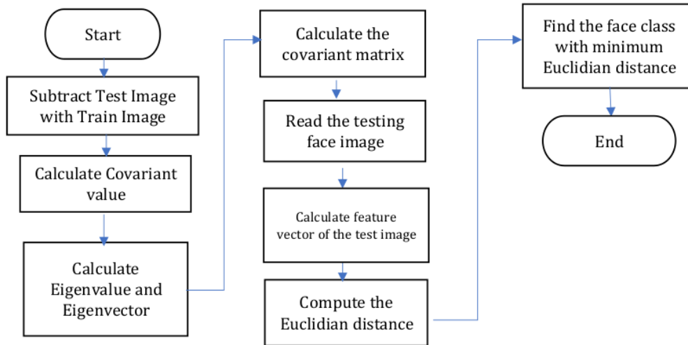
Figure 2. The Flowchart of PCA
