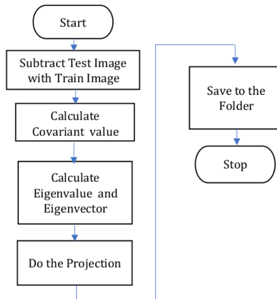
Figure 1. The steps involved in eigenface method
