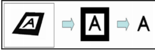
Gambar 8. Pattern Normalization dan Template Matching.
