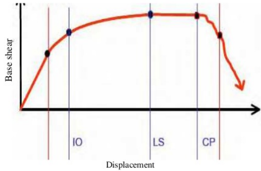
Fig. 1 Curve capacity
