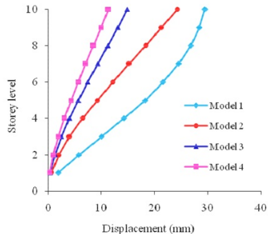
Fig. 5 Lateral displacements
