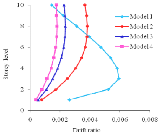
Fig. 6 Drift ratio
