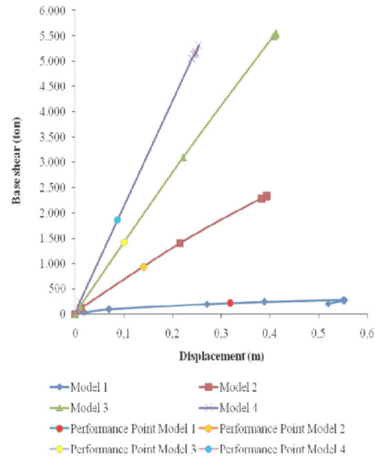
Fig. 7 Curve capacity
