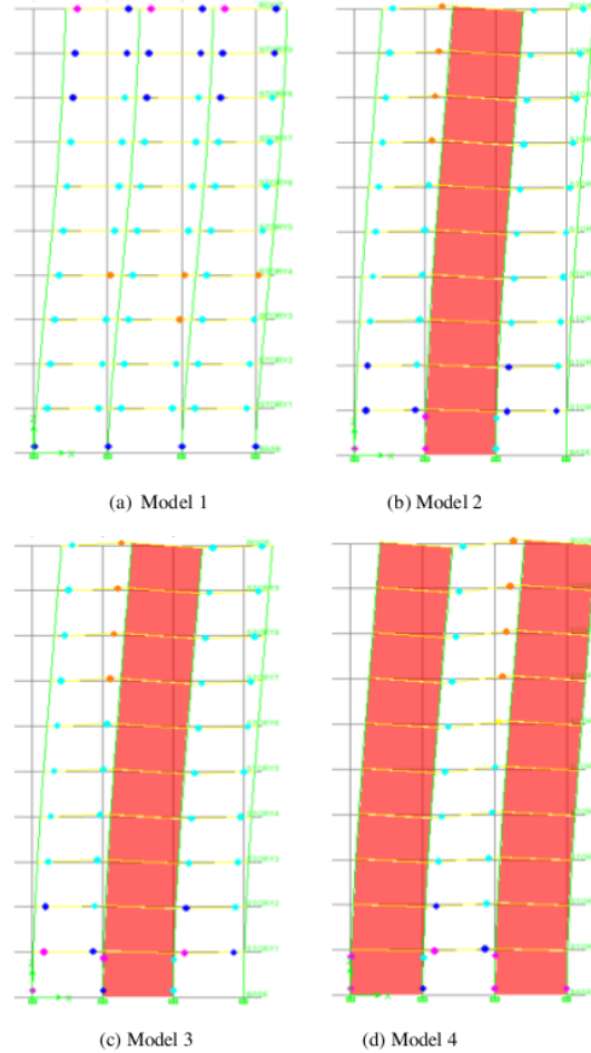
Fig. 10 The plastic hinges in the last step
