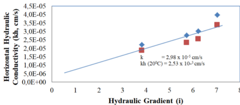
Figure 4: Horizontal hydraulic conductivity ( k_h ) versus hydraulic gradient ( i ) from Dusun III Banyu Urip sample
