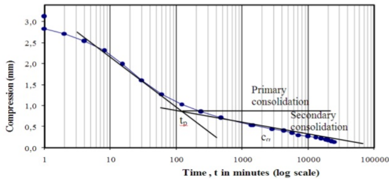
Figure 1: The time versus compression curves
