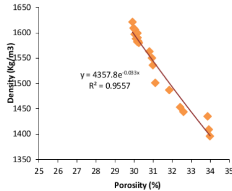
Figure 3.13. Relations porosity and density with the RHA 0%
