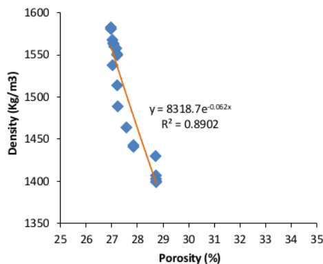
Figure 3.12. Relations porosity and density with the RHA 10%
