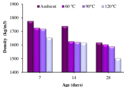
Figure 3 Density of foamed concrete without fly ash
