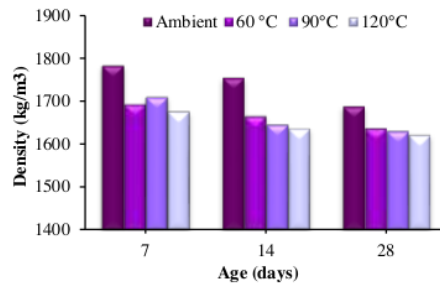
Figure 2 Density of foamed concrete with fly ash 10%
