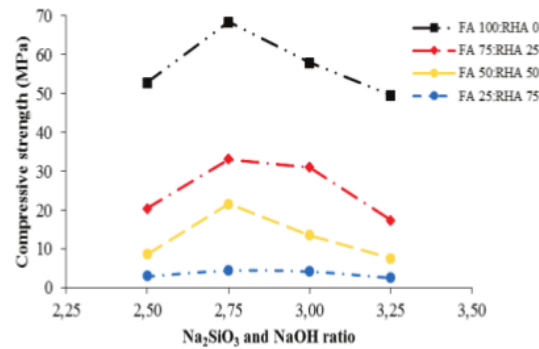
FIGURE 11. The effect of \text{Na}_2\text{SiO}_3 and NaOH ratio on compressive strength result of 28 days
