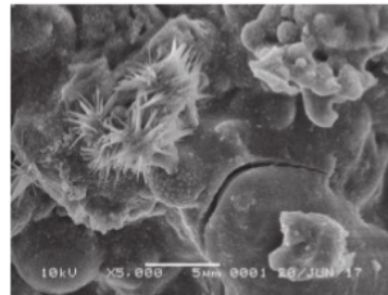
(a) \text{Na}_2\text{SiO}_3/\text{NaOH} 2.50
