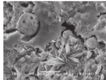
(b) \text{Na}_2\text{SiO}_3/\text{NaOH} 2.75
