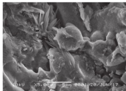
(a) \text{Na}_2\text{SiO}_3/\text{NaOH} 2.50
