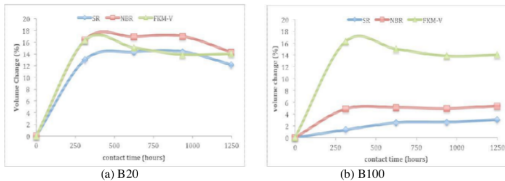
Figure 3. Profile change in O-rings volume during contact immersion time with B20 and B100.
