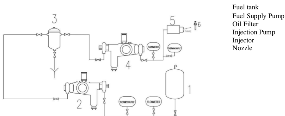
Figure 1. O-rings test apparatus (in Boiler Fuel System).
