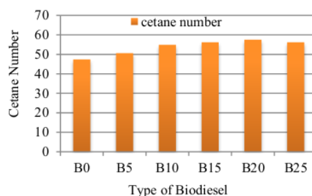
Fig. 6 The influence of Biodiesel Percentage to Cetane Number
