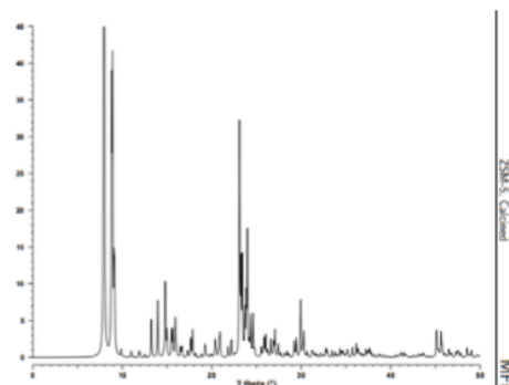
Figure 3. ZSM-5 Diffractogram Standard [23]
