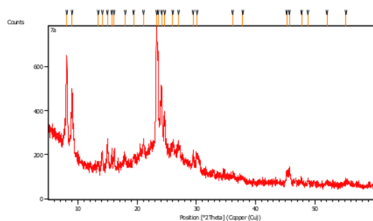
Figure 2. XRD ZSM-5 diffractogram
