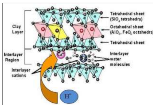
Fig 1: Bentonite reaction of HCl activation
