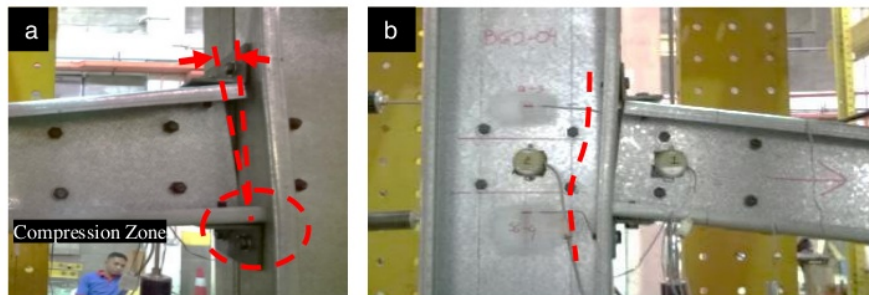
Figure 4. Deformation of specimen IJT-BGJ-4
