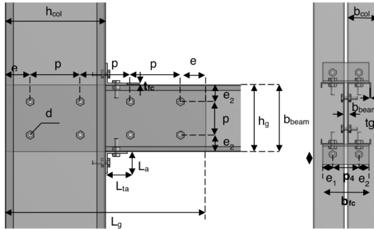
Figure 1. Detail of specimen
