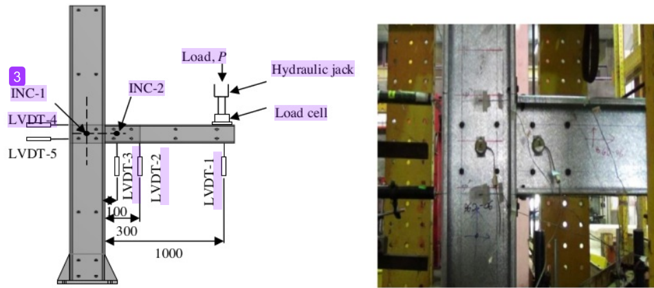
Figure 3. Testing of Specimen with Isolated Joint Test (IJT)
