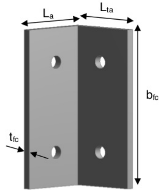
Figure 2. Dimension of flange cleat
