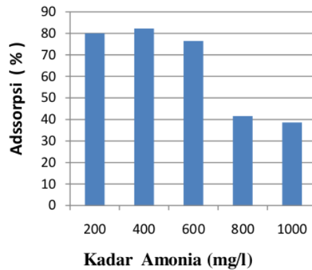
Gambar 4. Pengaruh kadar amonia terhadap adsorpsi bentonit
