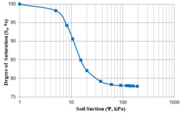
Fig. 6. Graph of saturation and suction degree of peat soil on the W5 sample
