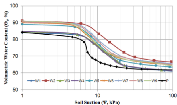
Fig. 10. Suction graph with volumetric water content due to wetting and drying influence on all peat soil samples
