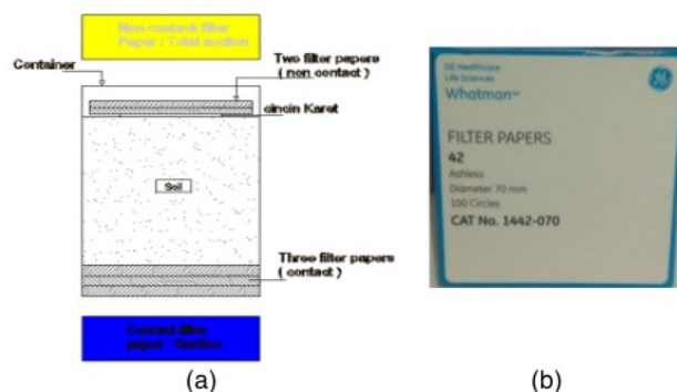
Fig. 3. Filter paper test
