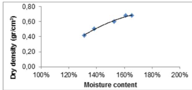
Fig. 7. The compaction (standard Proctor) test results.
