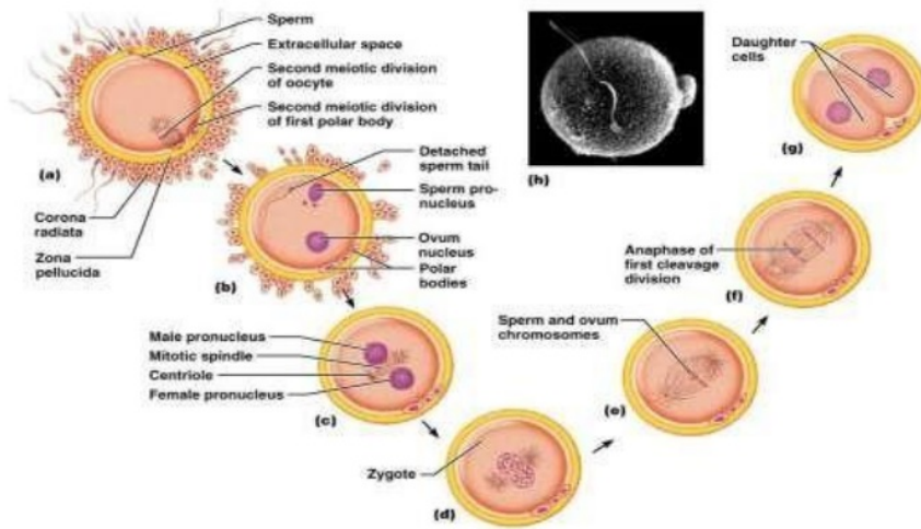
Figure 5. Fertilization Process
