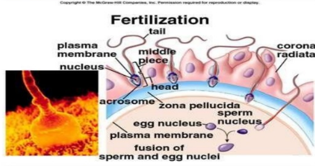
Figure 1. Fertilization
