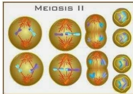
Figure 14. Meiosis II
