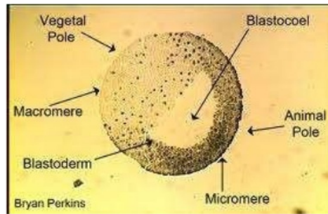
Figure 19. Blastula Cells
