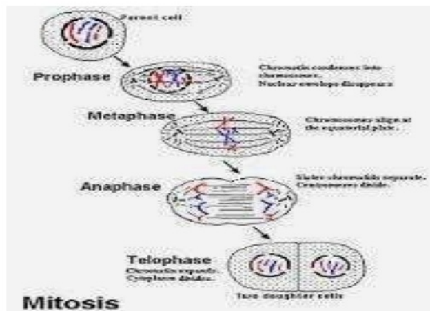
Figure 7. Mitotic Cleavage
