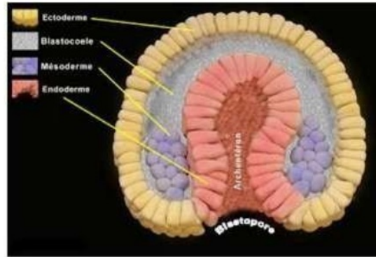
Figure 20. Gastrula Cells
