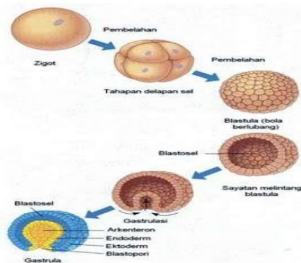
Figure 16. Cleavage
