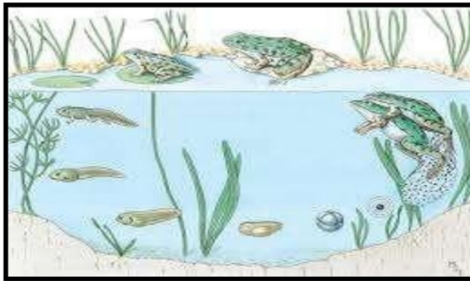
Figure 2. External fertilization
