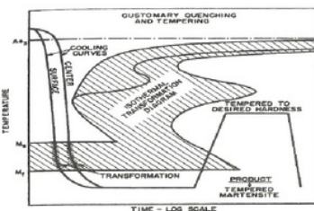
Gambar 5. Proses Quenching dan Tempering
