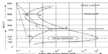
Gambar 4. Temperature Transformation
