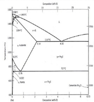
Gambar 1. Diagram Fasa Fe-Fe 3 C
