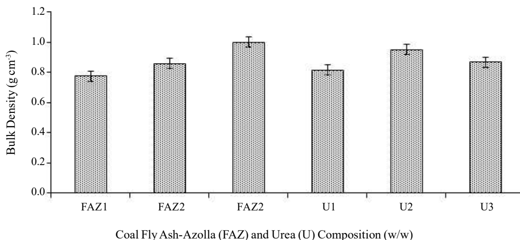
Figure 2. Bulk density of the briquette fertilizers with various proportion of coal fly ash-azolla (FAZ) and urea (U).
