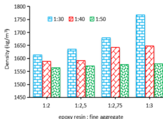
Fig 4. Effect of percentage of epoxy and fine aggregate on the density
