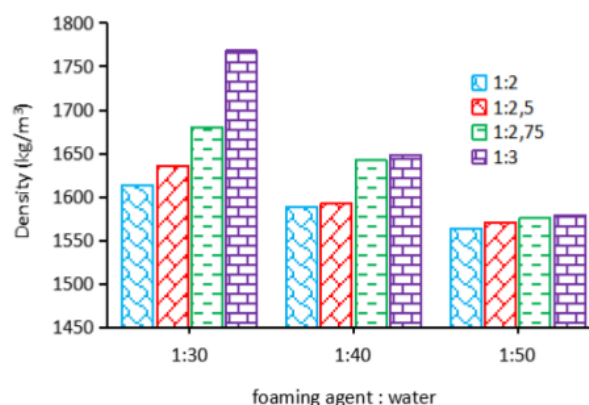
Fig 5. Effect of percentage foaming agent and water on specific gravity
