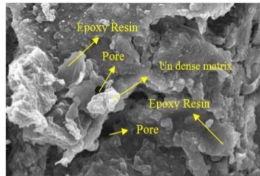
Fig 8. Microstructure test results in immersion \text{Al}_2\text{SO}_4
