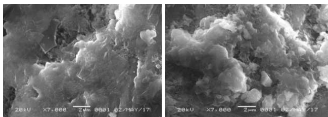
(a) w/c = 0.275
