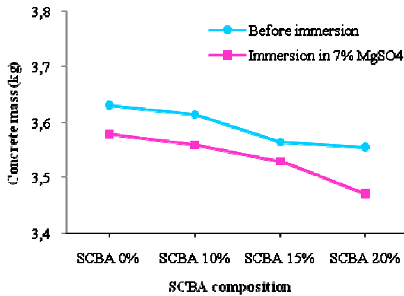
Fig. 10 The effect of SCBA content on concrete mass with w/c = 0.325 ( \text{MgSO}_4 = 7\% )
