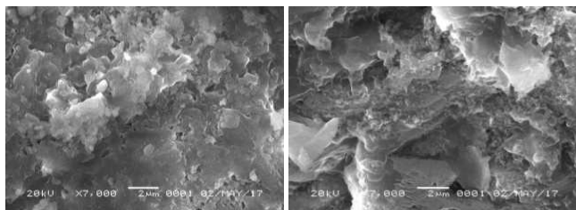
(a) w/c = 0.275
