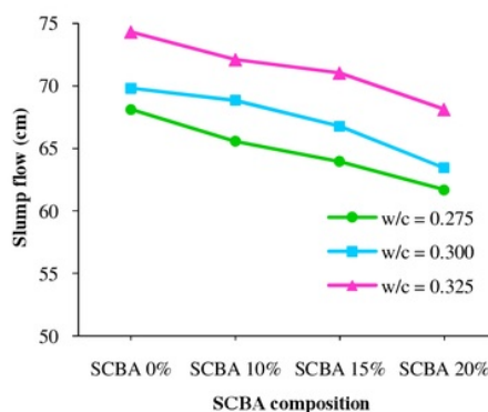
1 Fig. 2 The effect of SCBA on slump flow
