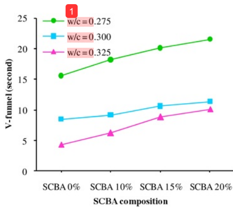
Fig. 3 The effect of SCBA on V-funnel
