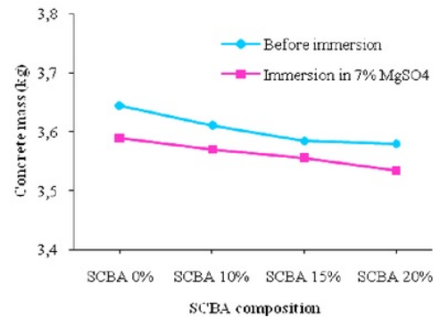
Fig. 9 The effect of SCBA content on concrete mass with w/c = 0.300 ( MgSO_4 = 7\% )
