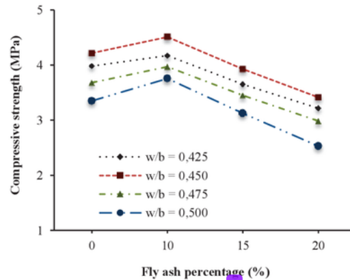
FIGURE 9. The effect of fly ash percentage on compressive strength at 28 days
