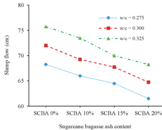
FIGURE 6. The effect of sugarcane bagasse ash on slump flow
