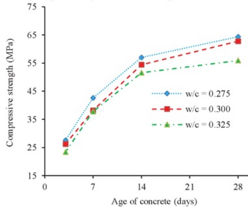
FIGURE 12. The effect of age of concrete on SCBA 10% compressive strength
