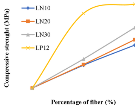
Figure 3. Compressive strength at age 28 days
