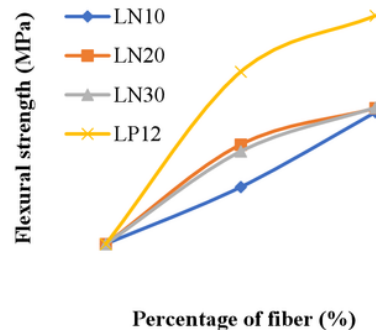
Figure 4. Strength flexural at age 28 days
