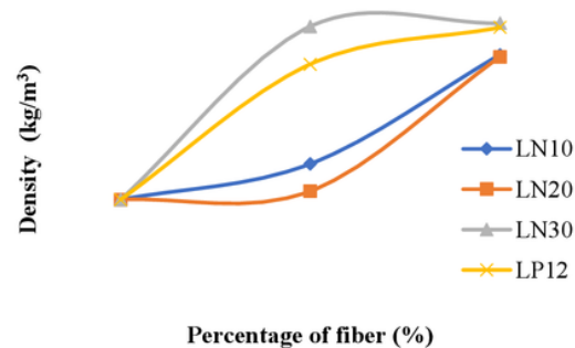
Figure 2. Density at age 28 days
