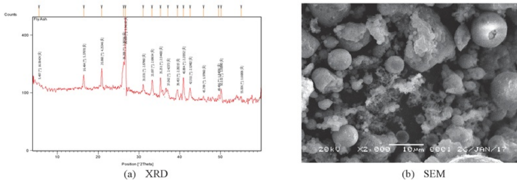
FIGURE 1. XRD and SEM fly ash test results
