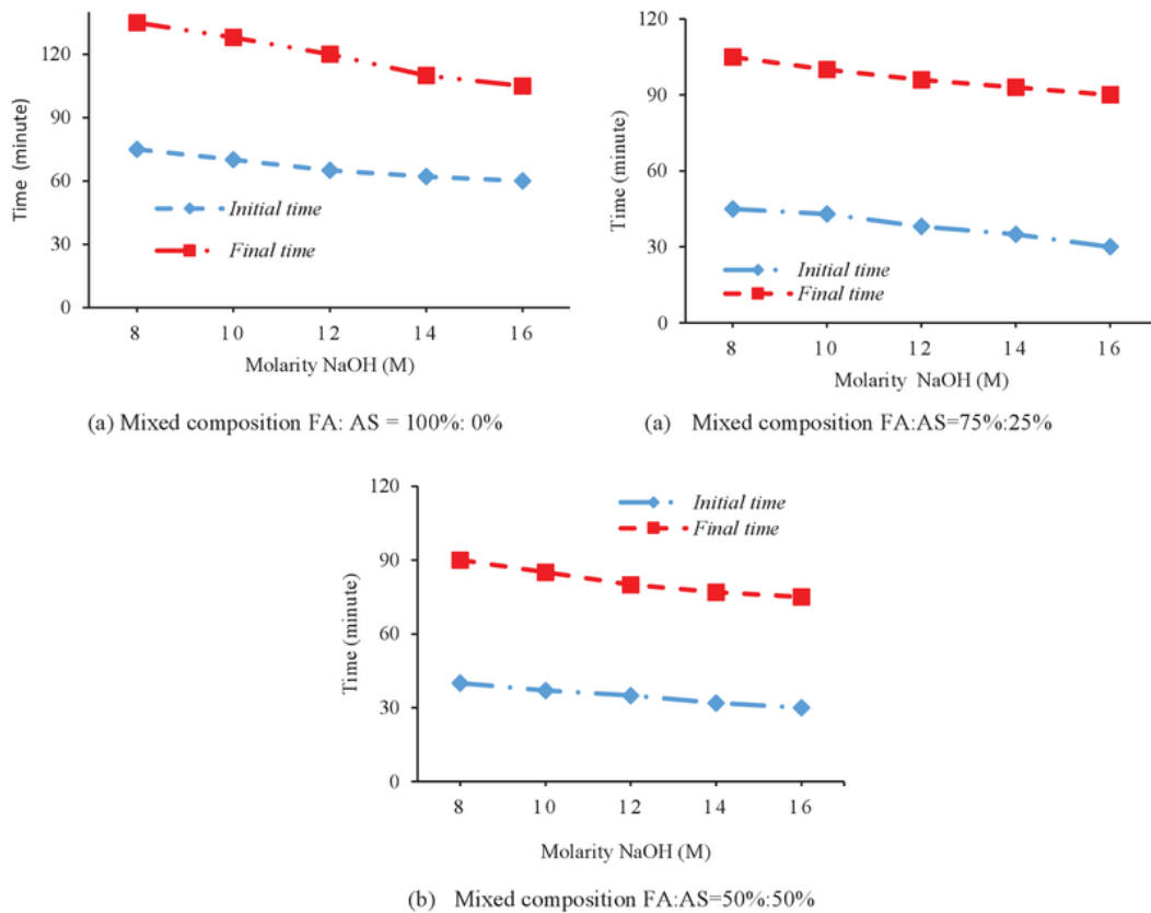
FIGURE 4. The result of the geopolymer mortar time setting test
