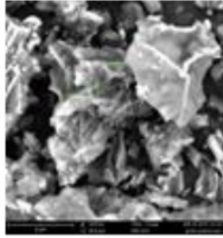
Figure 5 SEM of Peat
