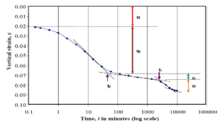
Figure 3 Consolidation behavior of peat
