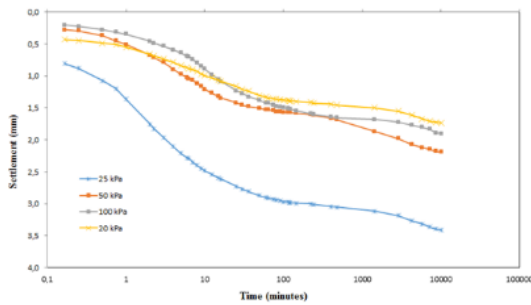
Figure 8 Time settlement curve from oedometer test
