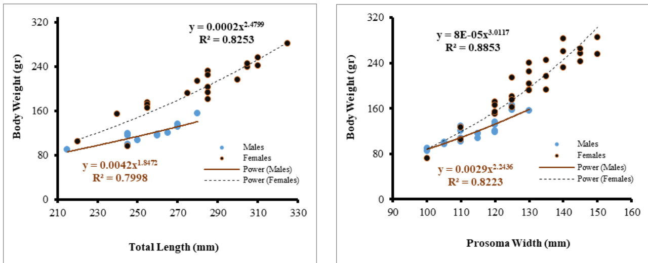
Figure 4. Total length-body weight (left) and prosoma width-body weight (right) relationship of males and females Carcinoscorpius rotundicauda from Banyuasin estuarine of South Sumatra, Indonesia. Both sex indicated the body weight grown slowly with respect to the total length (negative allometric, b < 3 , p < 0.05 ) while the body weight of females also grown slowly with respect to the prosoma width (negative allometric, b < 3 , p < 0.05 ) but the prosoma width and body weight for males grown at the same rate (isometric, b = 3 , p < 0.05 ).
