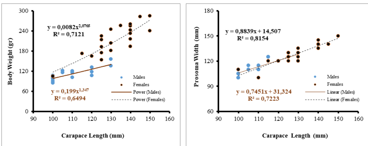
Figure 5. Carapace length-body weight (left) and prosoma width-carapace length (right) relationship of males and females Carcinoscorpius rotundicauda from Banyuasin estuarine of South Sumatra, Indonesia. The body weight grew slowly with respect to the carapace length (negative allometric, b < 3 , p < 0.05 ) for both sexes while the carapace length and prosoma width grown at the same rate (isometric, b = 1 , p < 0.05 ).
