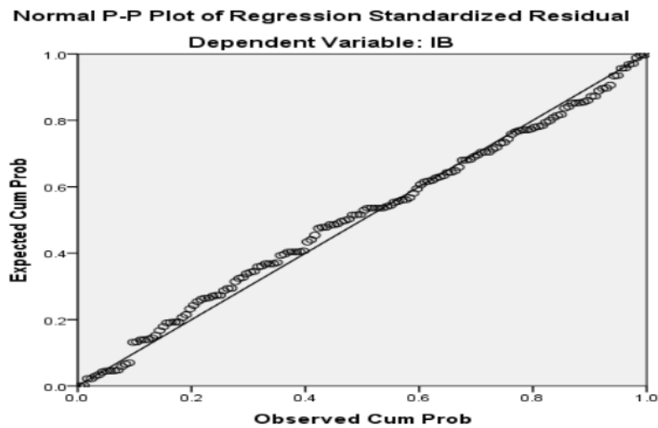
Figure 2: Normality Test
