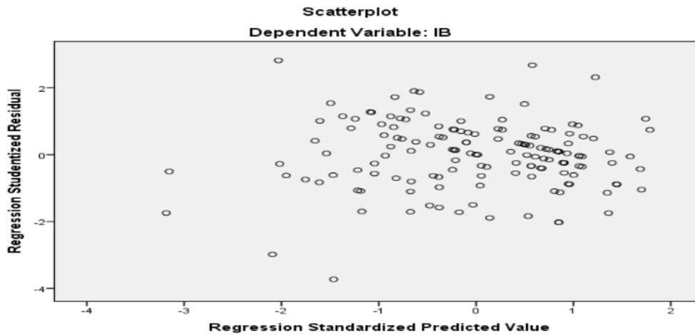
Figure 1: Heteroscedasticity Test
