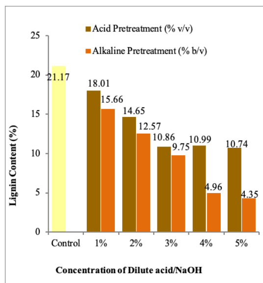
Figure 3. Effect of the Pretreatment on the Lignin Content of Rice Husk
