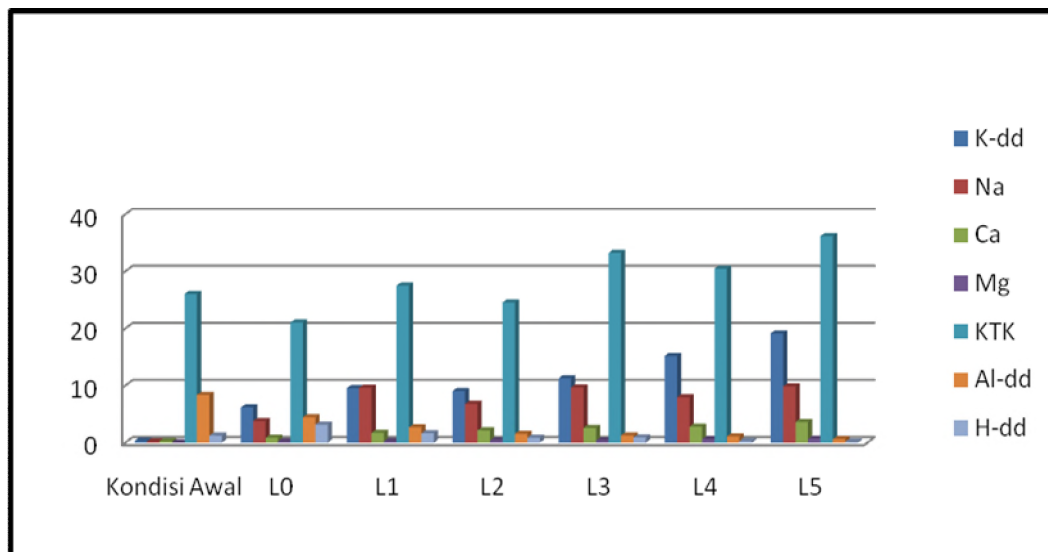
Figure 2. The change of soil K-dd, Na, Ca, Mg, CEC and Al-dd before and after applications of palm oil mill effluent.
