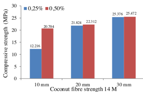
Fig 3. Length and Compressive Strength 14M
