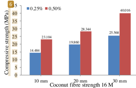
Fig 4. Fibre Length and Compressive Strength 16M
