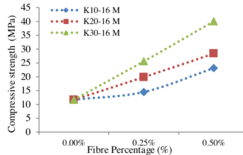
Fig 2. Fibre (%) and Compressive Strength
