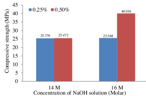
Figure 5. Molarity and Compressive Strength
