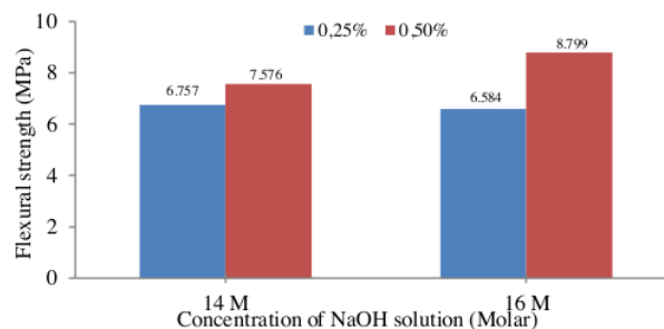
Figure 10. Molarity and Flexural Strength
