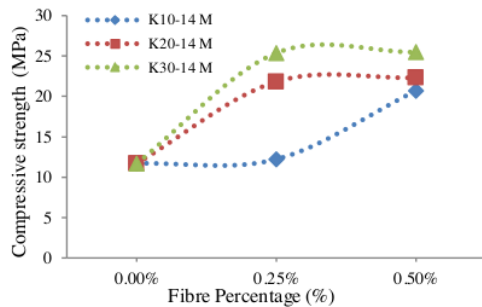
Fig 1. Fibre (%) and Compressive Strength 14M
