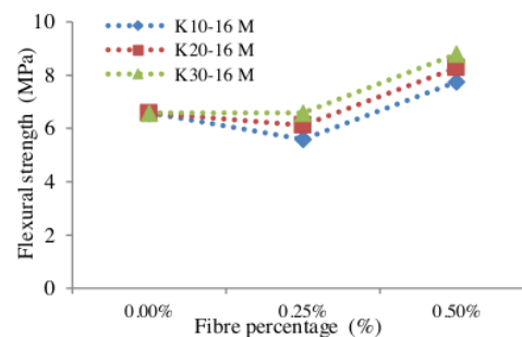
Fig 7. Fibre (%) and Flexural Strength 16M
