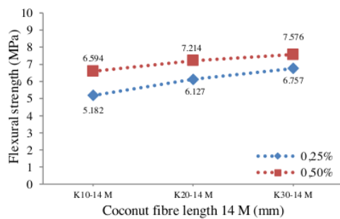
Fig 8. Fibre and Flexural Strength 14M
