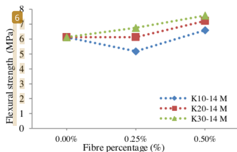
Fig 6. Fibre (%) and Flexural Strength 14M
