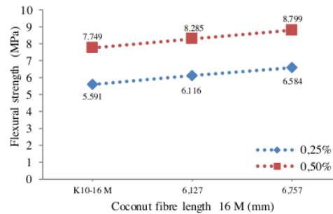
Fig 9. Fibre and Flexural Strength 16M
