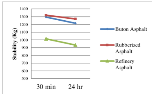
Figure 4. Retained strength index for thin SMA
