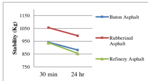
Figure 6. Retained strength index for rough SMA
