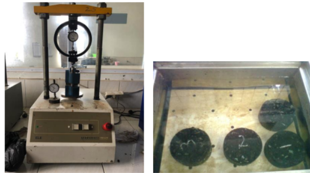
Figure 2. Marshall machine and Sample soaked in waterbath
