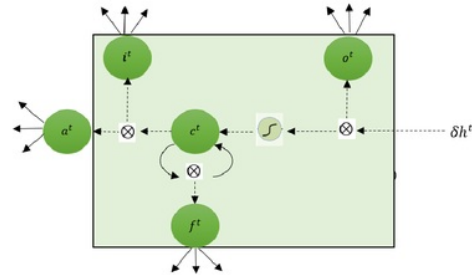
Fig. 4. Backward pass in LSTM
